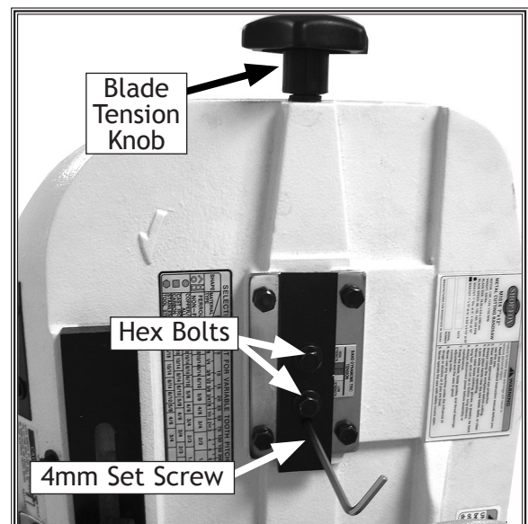
Figure 48. Tracking adjustment controls.
